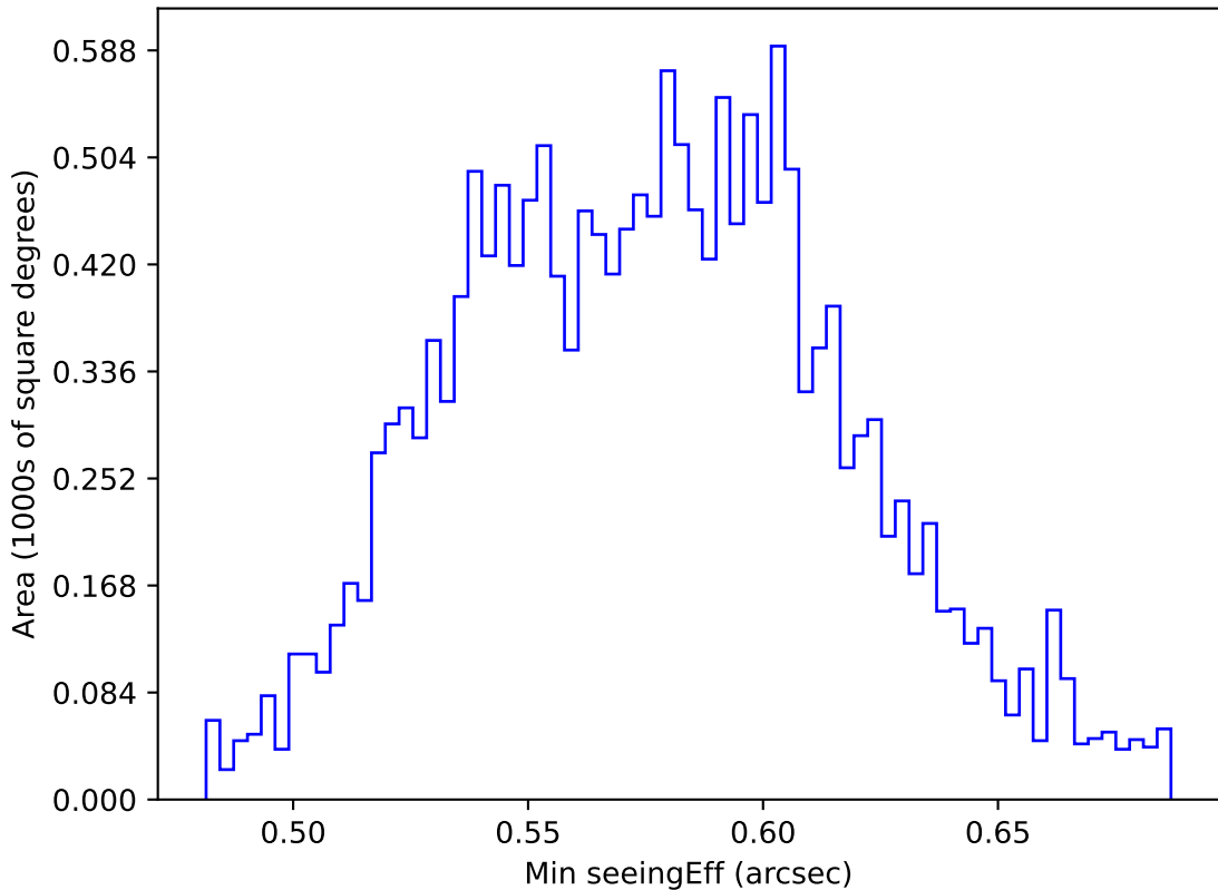
internal_u_expt45_nscale1.2v3.4_10yrs WFD all bands: Min seeingEff
