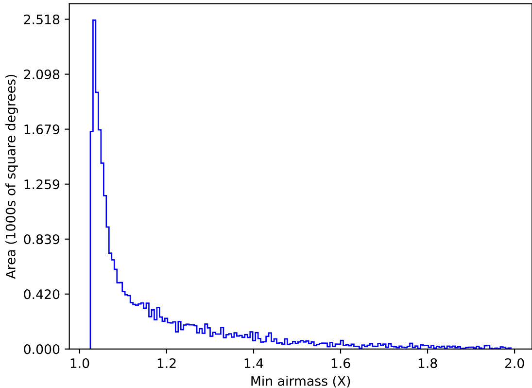
internal_u_expt45_nscale1.2v3.4_10yrs Yr 1 z band: Min airmass
