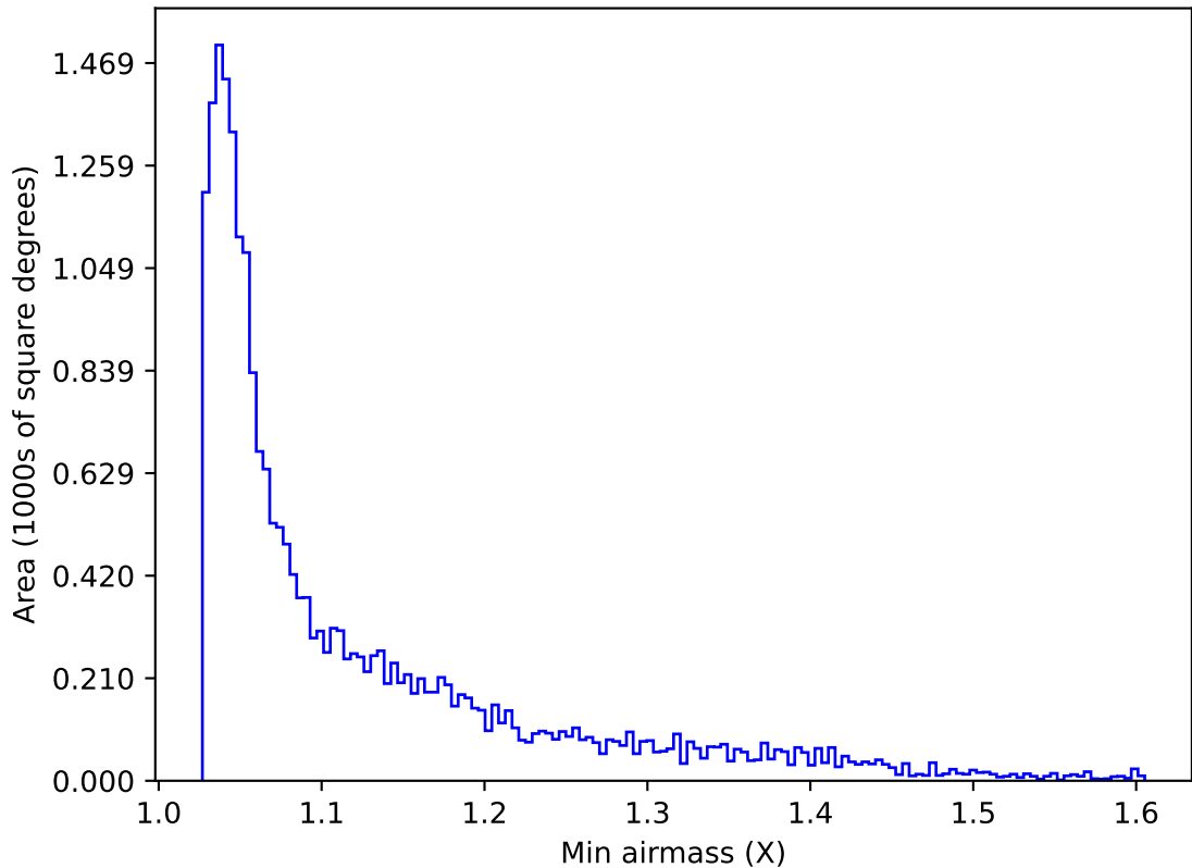
internal_u_expt45_nscale1.2v3.4_10yrs Yr 1 y band: Min airmass
