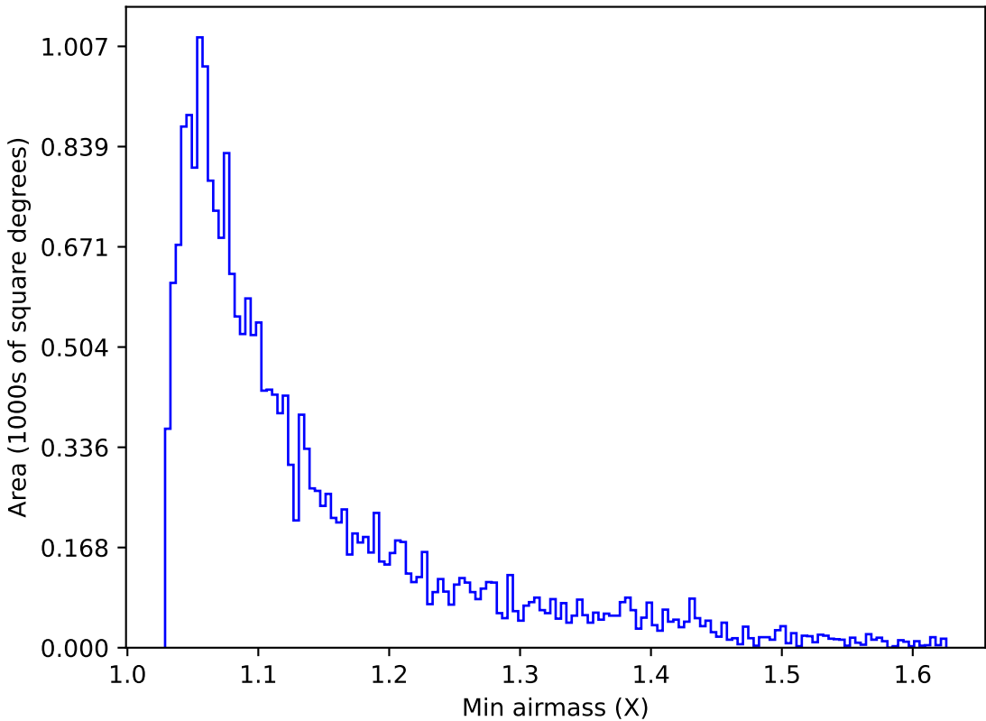
internal_u_expt45_nscale1.2v3.4_10yrs Yr 1 u band: Min airmass
