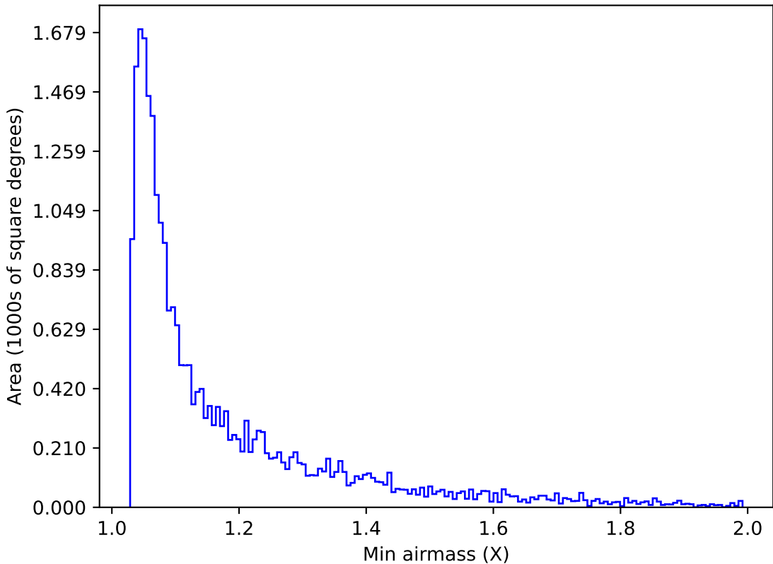
internal_u_expt45_nscale1.2v3.4_10yrs Yr 1 g band: Min airmass
