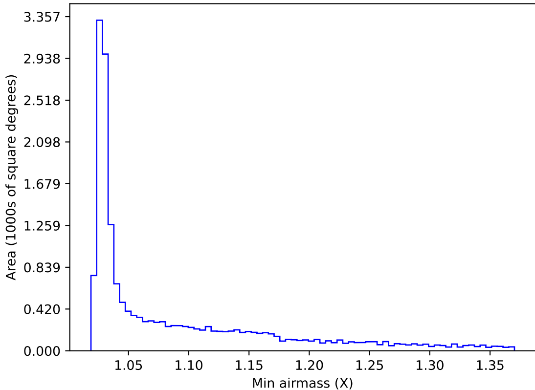
internal_u_expt45_nscale1.2v3.4_10yrs WFD z band: Min airmass
