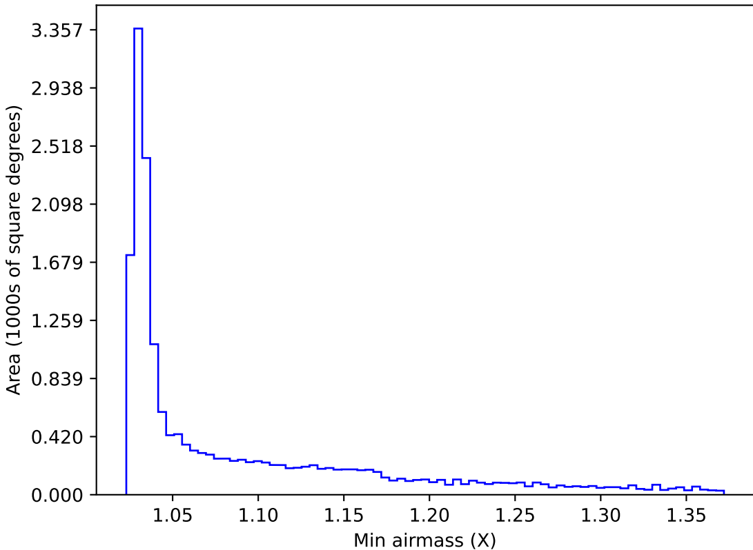
internal_u_expt45_nscale1.2v3.4_10yrs WFD y band: Min airmass
