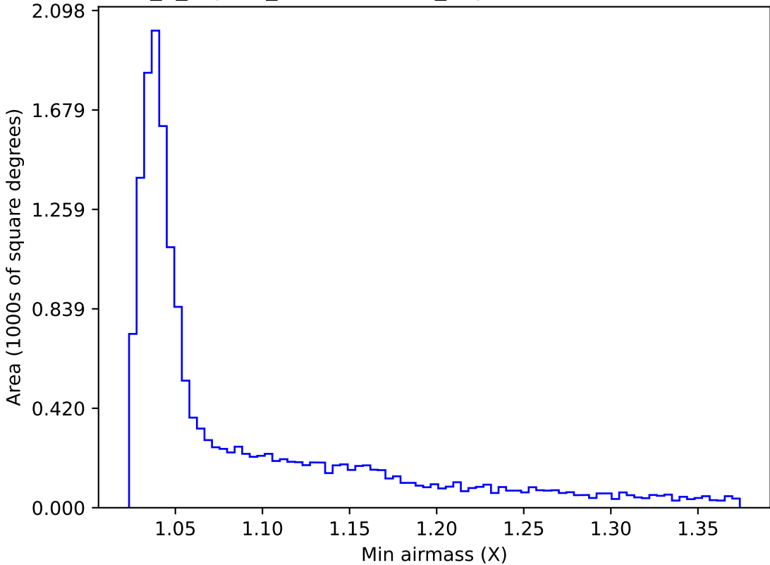
internal_u_expt45_nscale1.2v3.4_10yrs WFD u band: Min airmass
