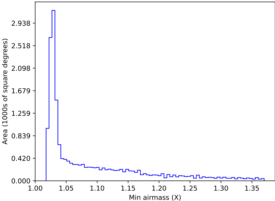
internal_u_expt45_nscale1.2v3.4_10yrs WFD i band: Min airmass
