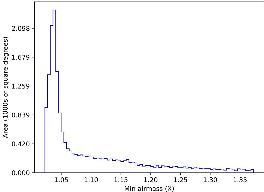
internal_u_expt45_nscale1.2v3.4_10yrs WFD g band: Min airmass
