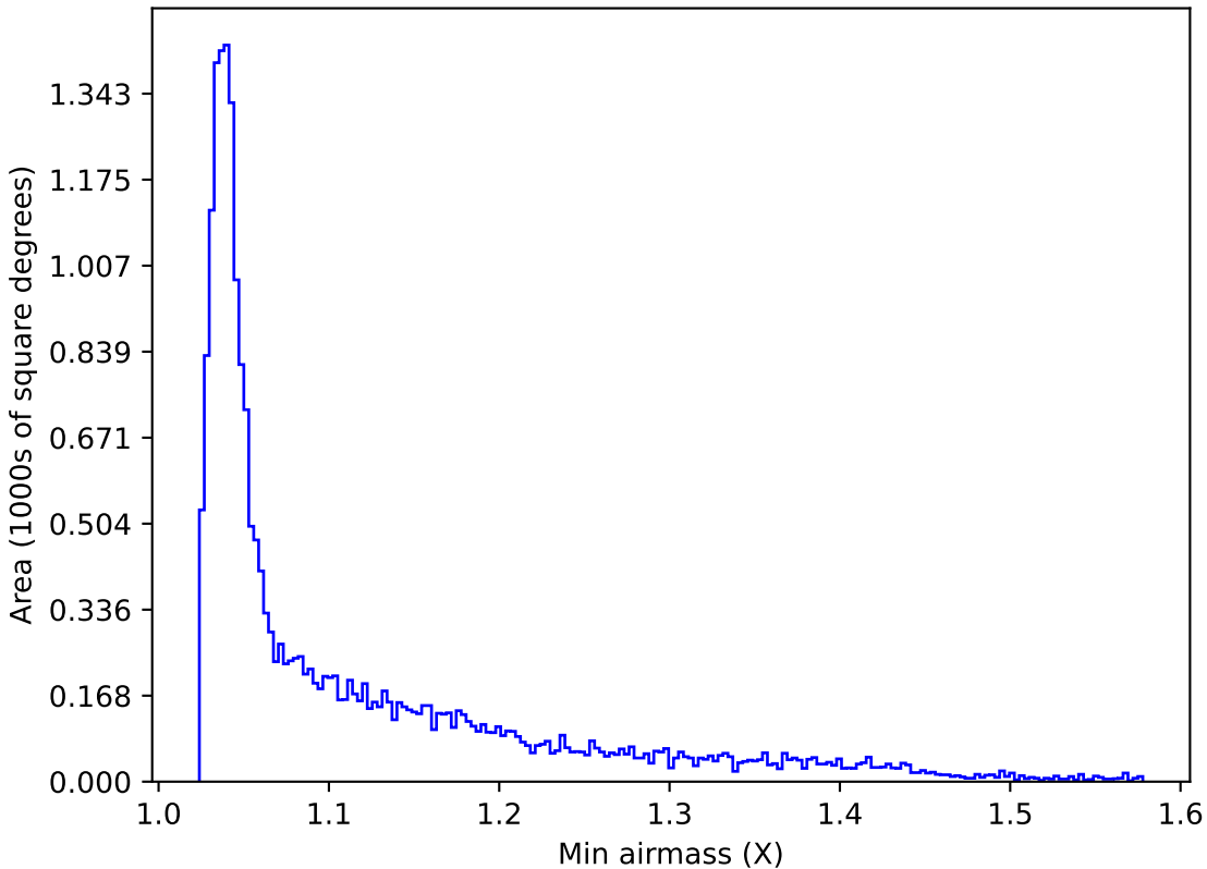
internal_u_expt45_nscale1.2v3.4_10yrs All sky u band: Min airmass
