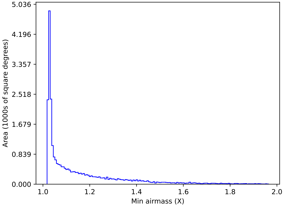
internal_u_expt45_nscale1.2v3.4_10yrs All sky r band: Min airmass
