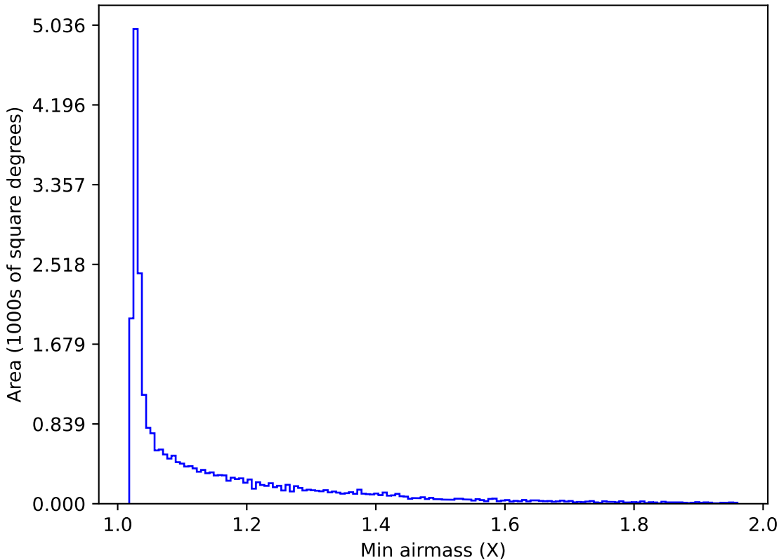
internal_u_expt45_nscale1.2v3.4_10yrs All sky i band: Min airmass
