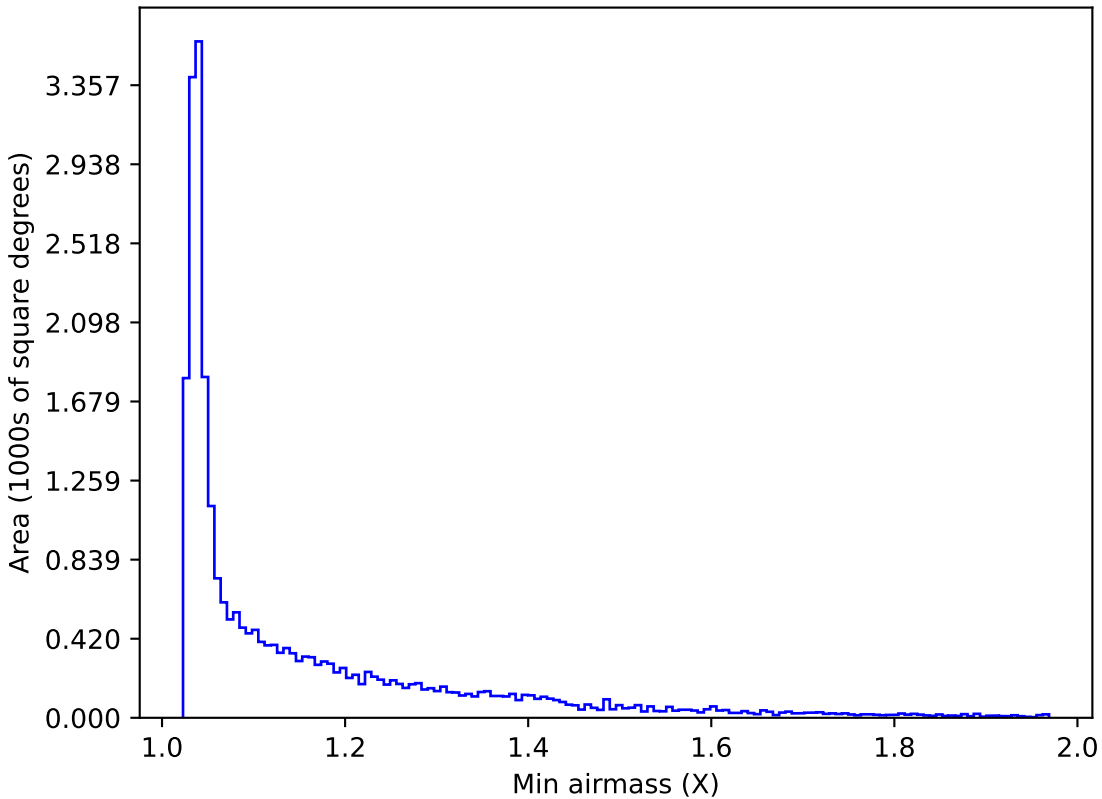
internal_u_expt45_nscale1.2v3.4_10yrs All sky g band: Min airmass
