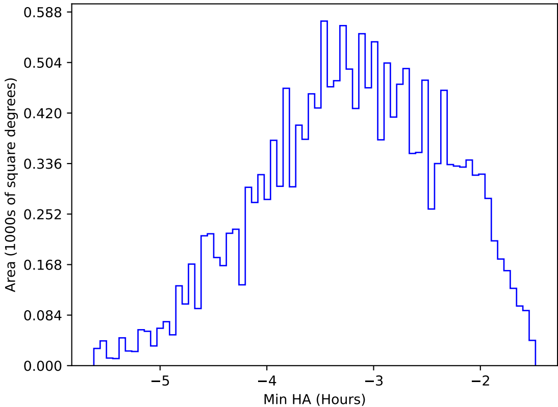
internal_u_expt45_nscale1.2v3.4_10yrs WFD u band: Min HA
