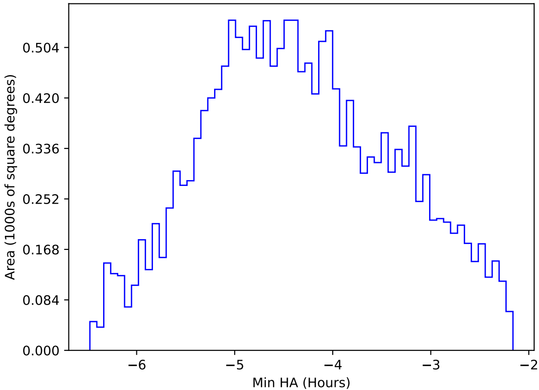
internal_u_expt45_nscale1.2v3.4_10yrs WFD i band: Min HA
