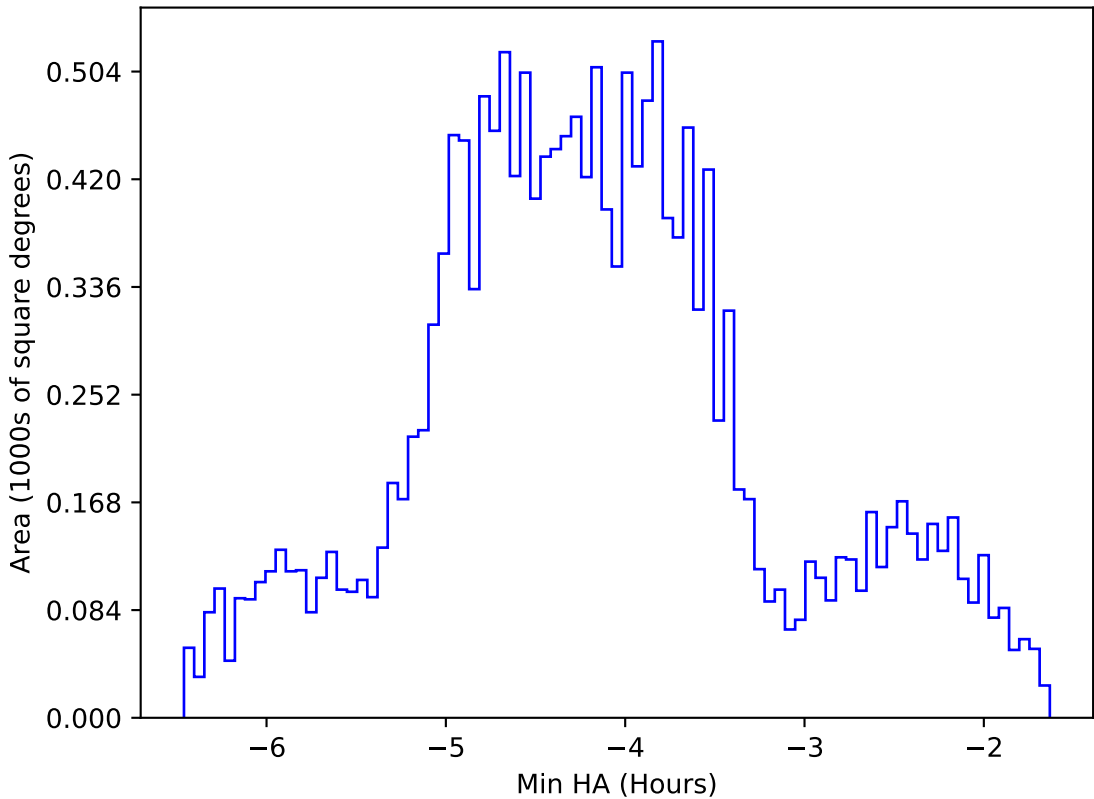
internal_u_expt45_nscale1.2v3.4_10yrs WFD g band: Min HA
