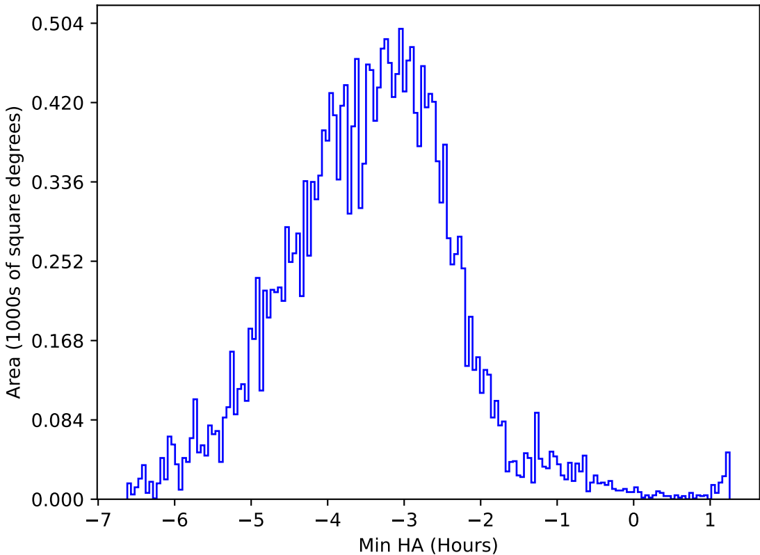
internal_u_expt45_nscale1.2v3.4_10yrs All sky y band: Min HA
