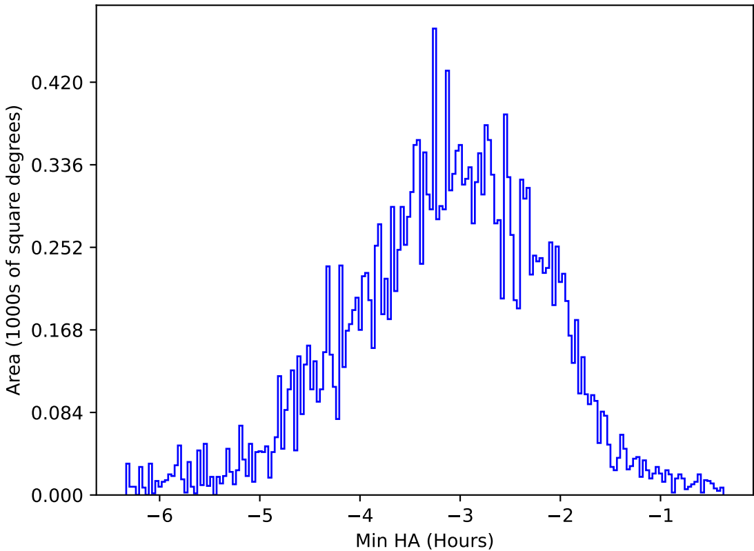
internal_u_expt45_nscale1.2v3.4_10yrs All sky u band: Min HA
