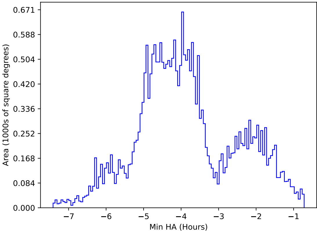
internal_u_expt45_nscale1.2v3.4_10yrs All sky g band: Min HA
