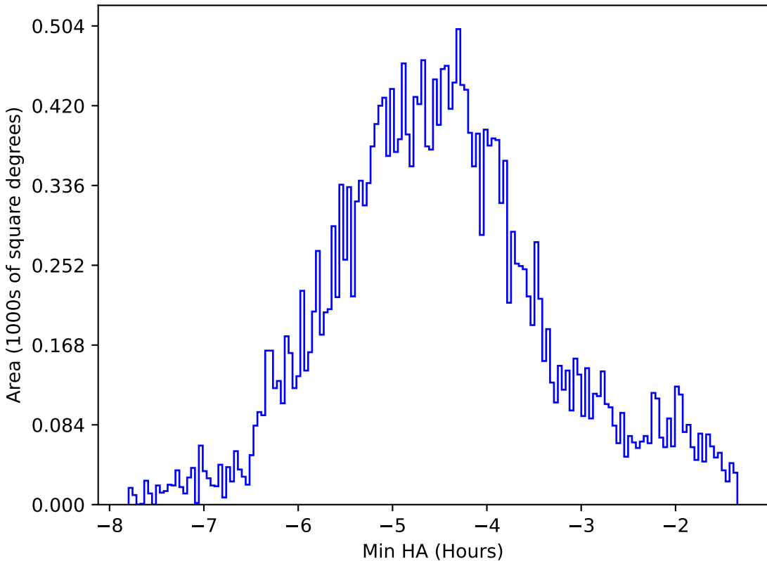
internal_u_expt45_nscale1.2v3.4_10yrs All sky all bands: Min HA
