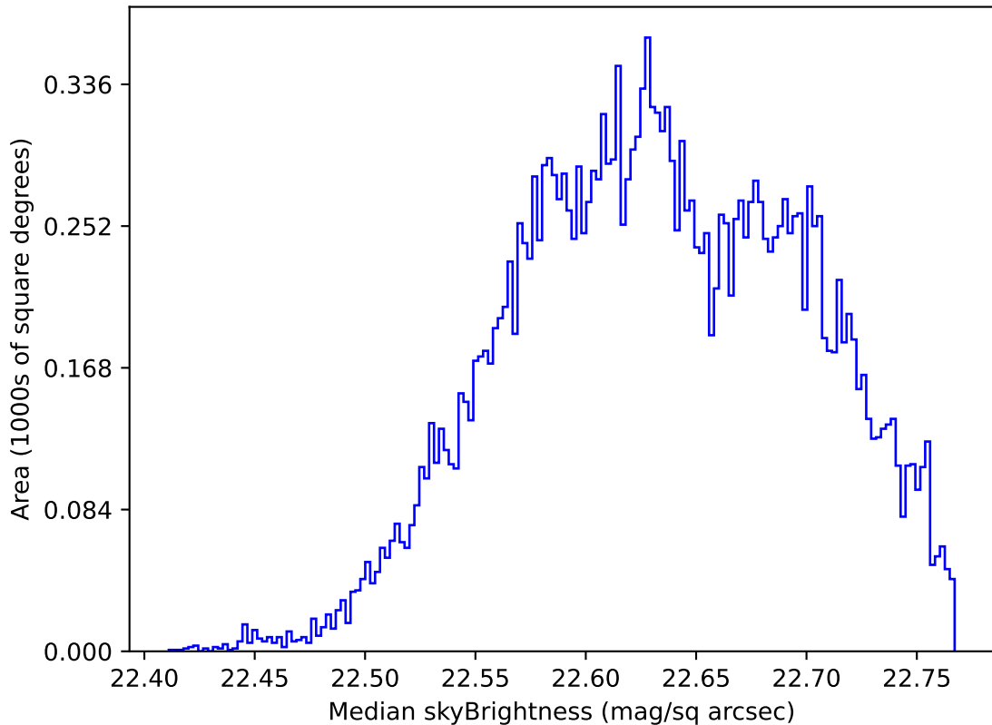
internal_u_expt45_nscale1.2v3.4_10yrs Yr 1 u band: Median skyBrightness
