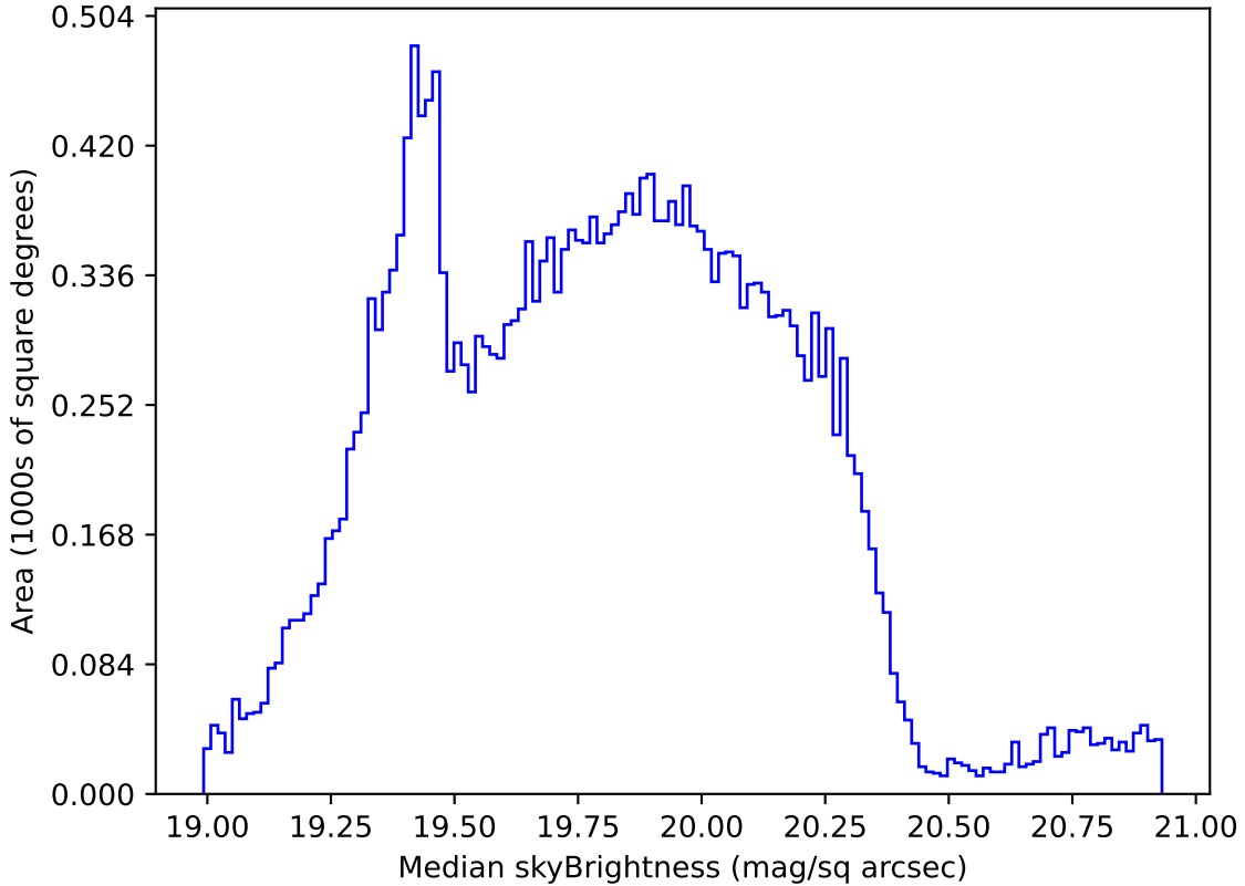
internal_u_expt45_nscale1.2v3.4_10yrs Yr 1 all bands: Median skyBrightness
