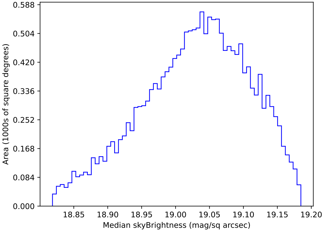
internal_u_expt45_nscale1.2v3.4_10yrs WFD z band: Median skyBrightness
