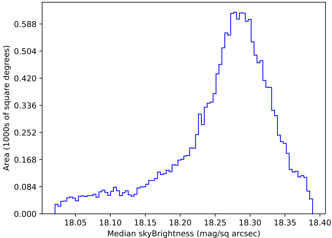
internal_u_expt45_nscale1.2v3.4_10yrs WFD y band: Median skyBrightness
