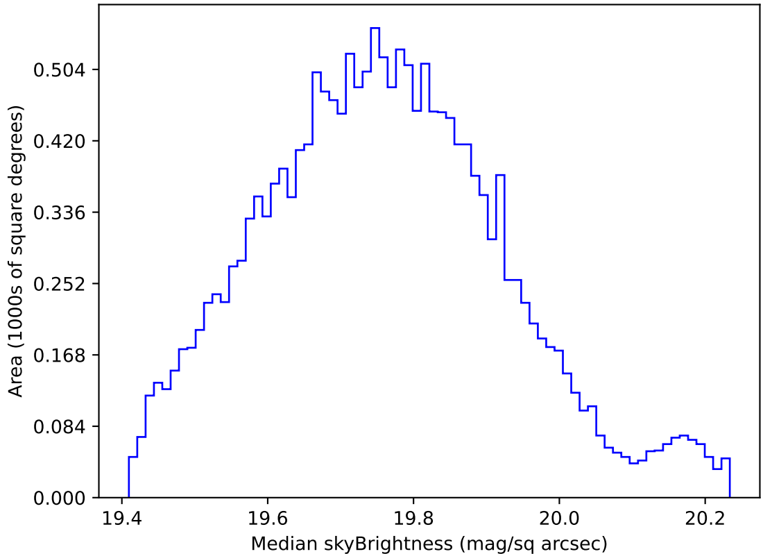
internal_u_expt45_nscale1.2v3.4_10yrs WFD all bands: Median skyBrightness
