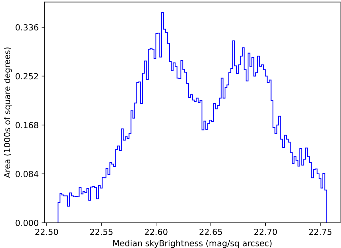
internal_u_expt45_nscale1.2v3.4_10yrs All sky u band: Median skyBrightness
