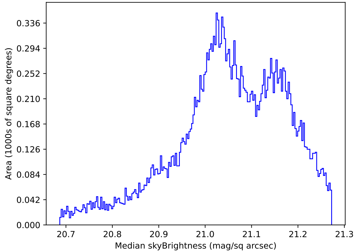
internal_u_expt45_nscale1.2v3.4_10yrs All sky r band: Median skyBrightness
