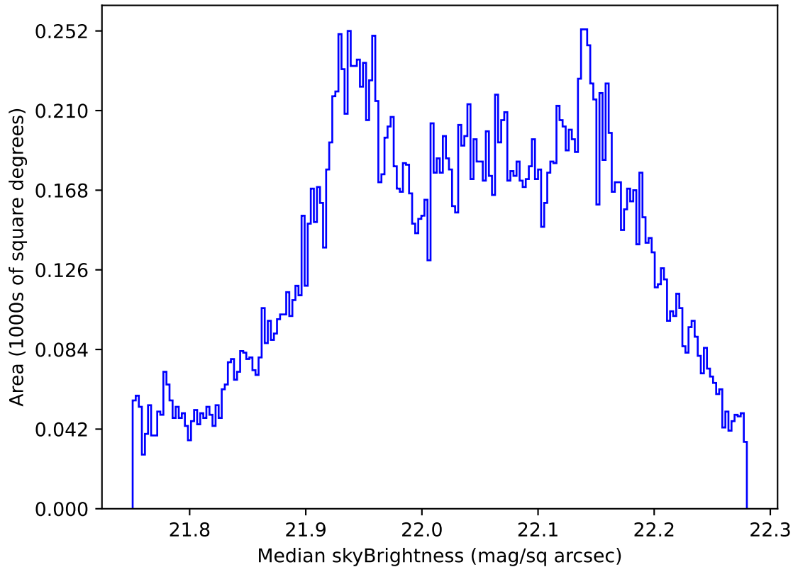
internal_u_expt45_nscale1.2v3.4_10yrs All sky g band: Median skyBrightness
