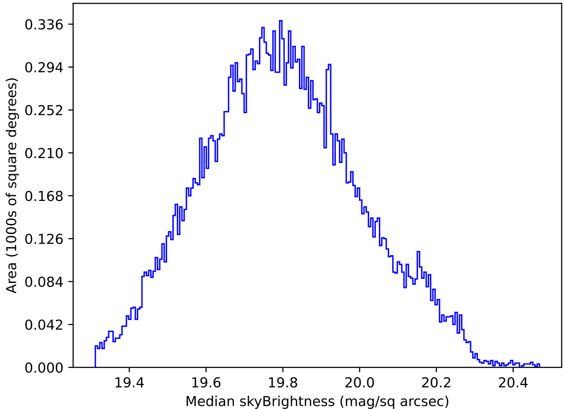
internal_u_expt45_nscale1.2v3.4_10yrs All sky all bands: Median skyBrightness
