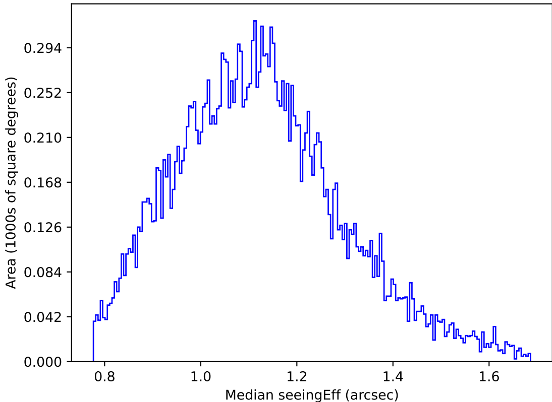
internal_u_expt45_nscale1.2v3.4_10yrs Yr 1 u band: Median seeingEff
