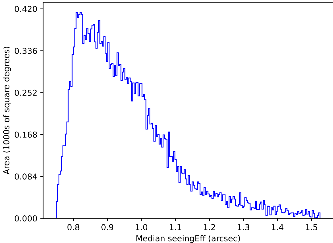
internal_u_expt45_nscale1.2v3.4_10yrs Yr 1 i band: Median seeingEff
