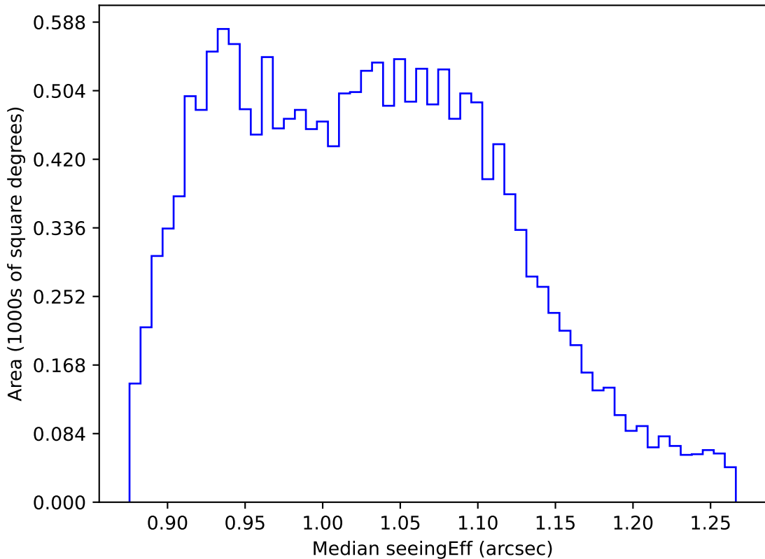
internal_u_expt45_nscale1.2v3.4_10yrs WFD r band: Median seeingEff
