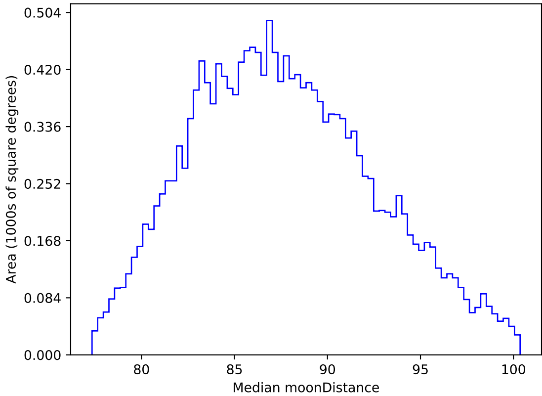
internal_u_expt45_nscale1.2v3.4_10yrs WFD all bands: Median moonDistance
