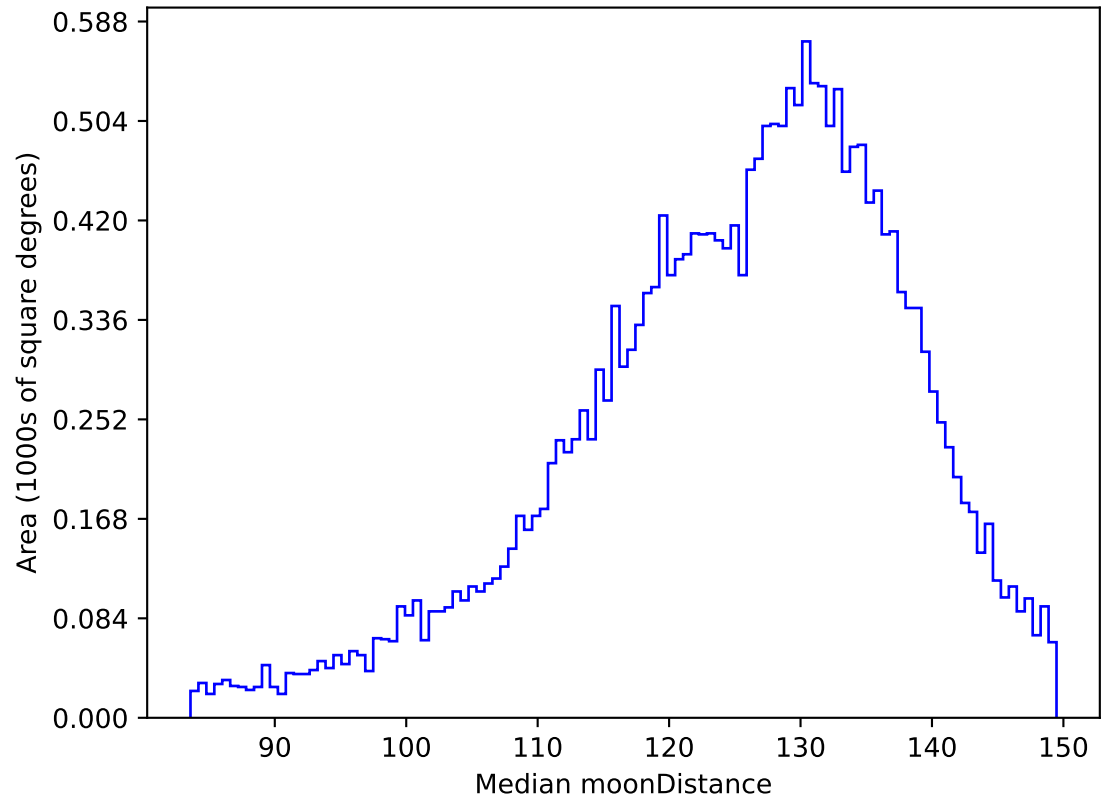
internal_u_expt45_nscale1.2v3.4_10yrs All sky u band: Median moonDistance
