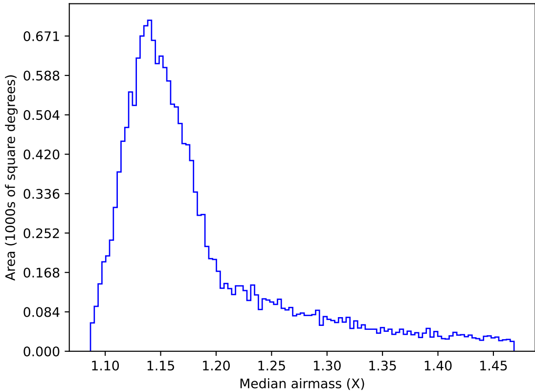
internal_u_expt45_nscale1.2v3.4_10yrs WFD z band: Median airmass
