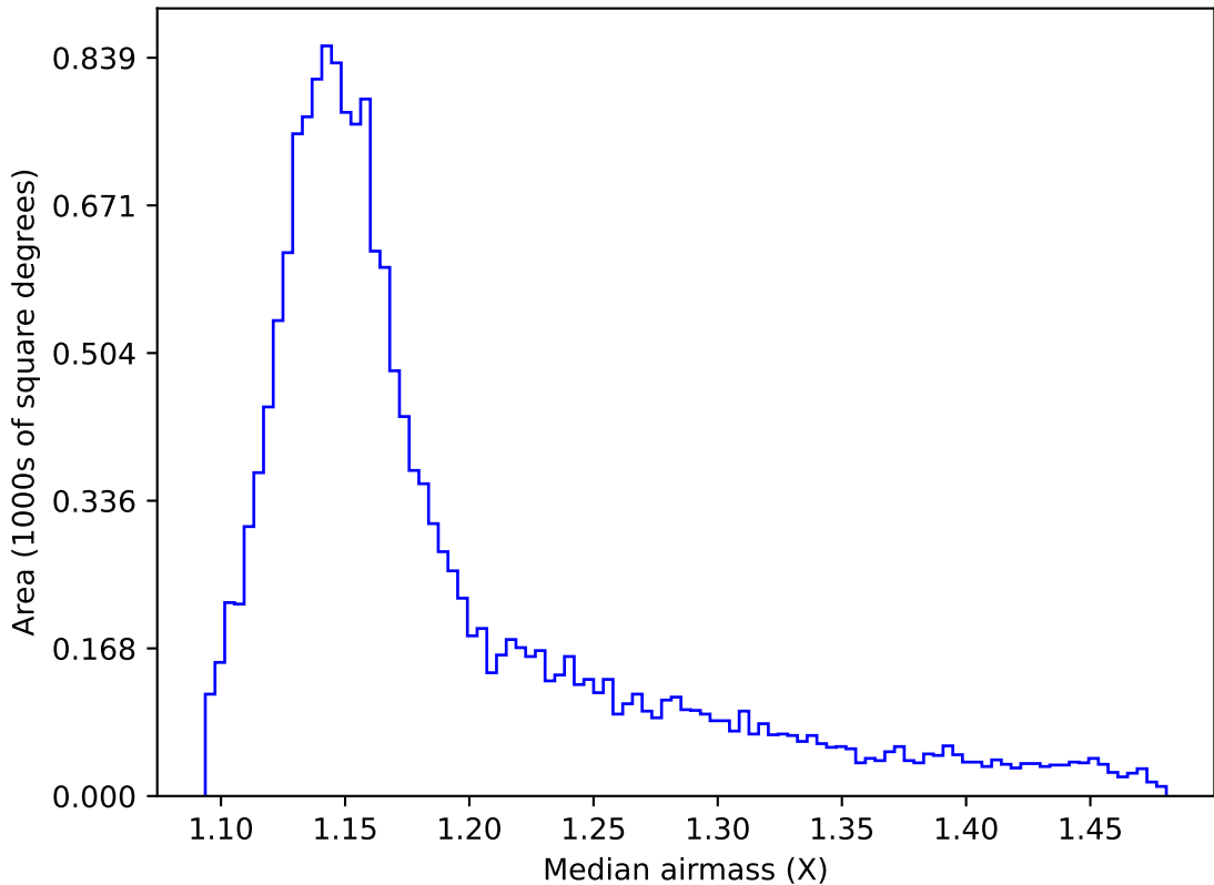
internal_u_expt45_nscale1.2v3.4_10yrs WFD y band: Median airmass
