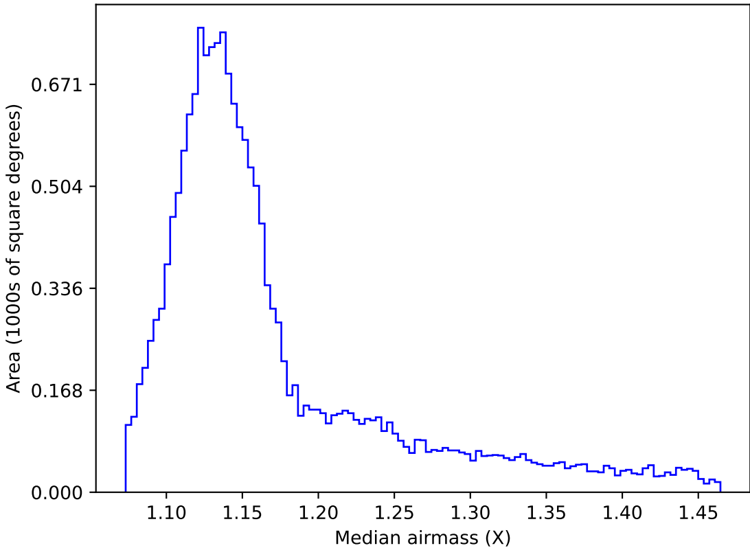
internal_u_expt45_nscale1.2v3.4_10yrs WFD r band: Median airmass
