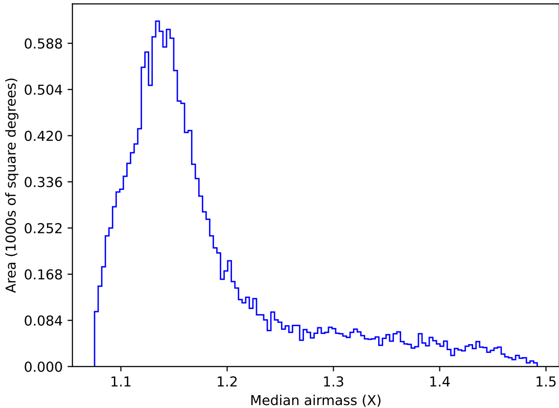
internal_u_expt45_nscale1.2v3.4_10yrs WFD g band: Median airmass
