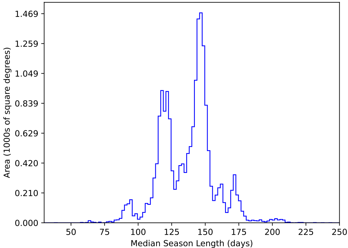
internal_u_expt45_nscale1.2v3.4_10yrs WFD y band: Median Season Length
