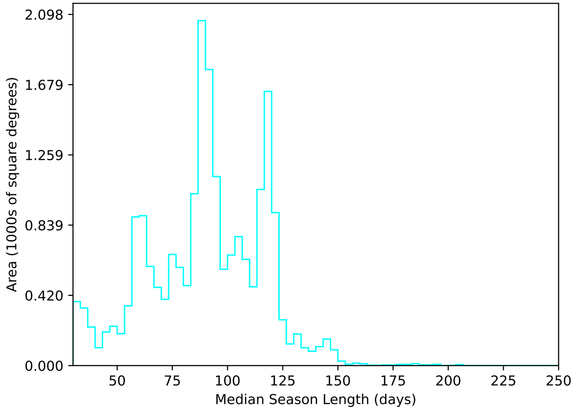
internal_u_expt45_nscale1.2v3.4_10yrs All sky u band: Median Season Length
