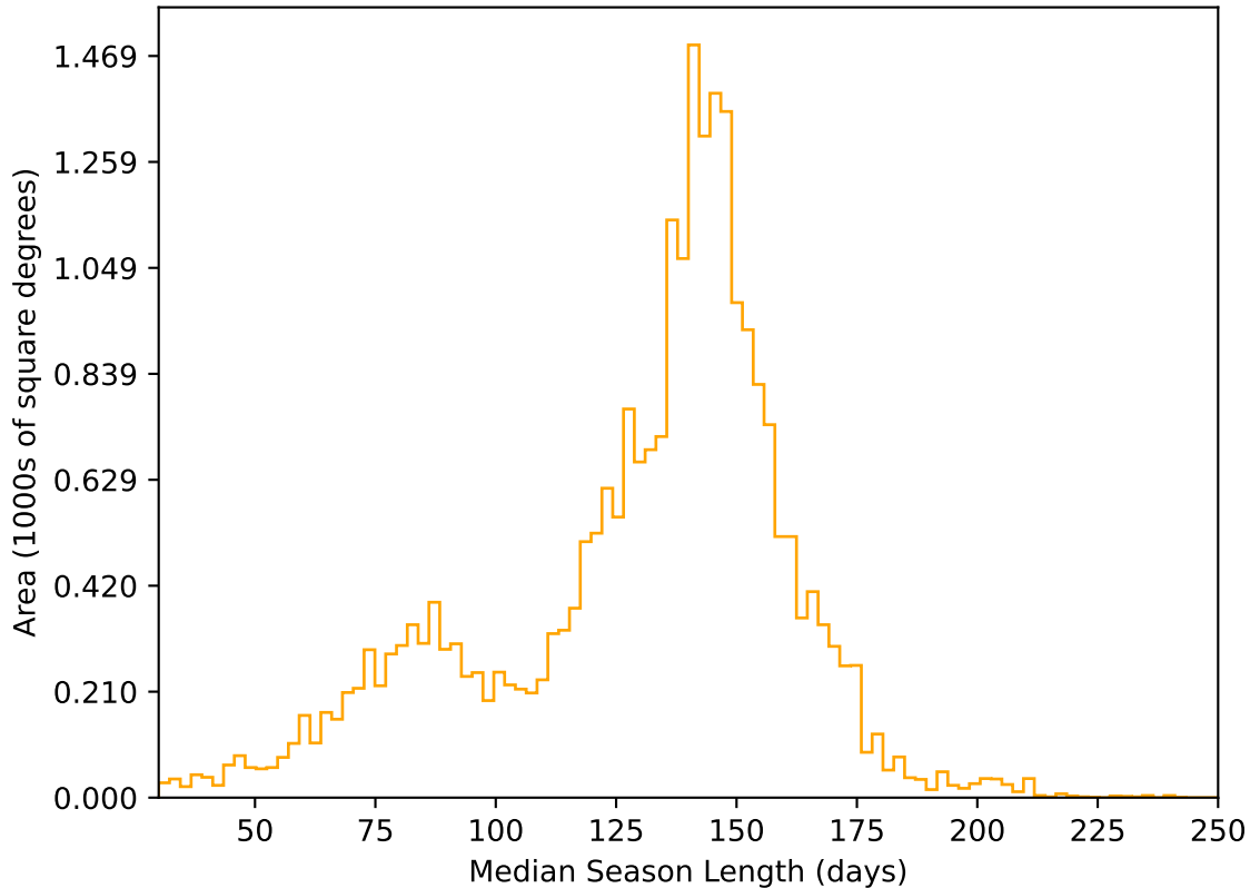
internal_u_expt45_nscale1.2v3.4_10yrs All sky r band: Median Season Length
