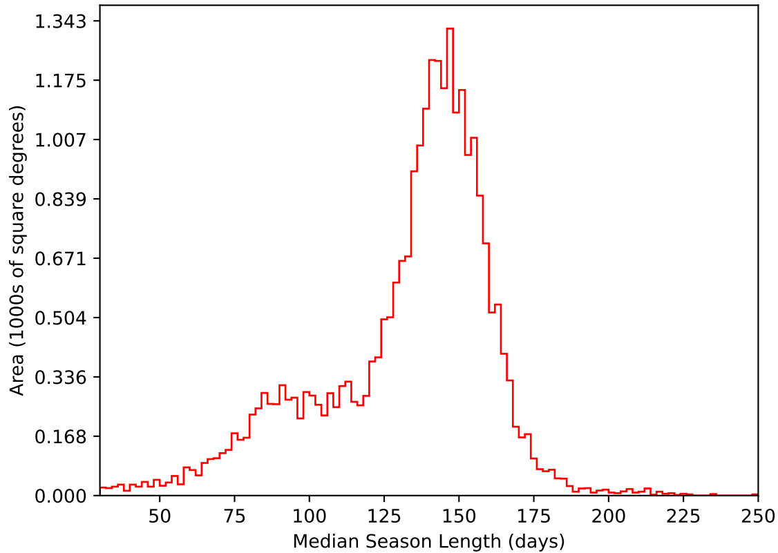
internal_u_expt45_nscale1.2v3.4_10yrs All sky i band: Median Season Length
