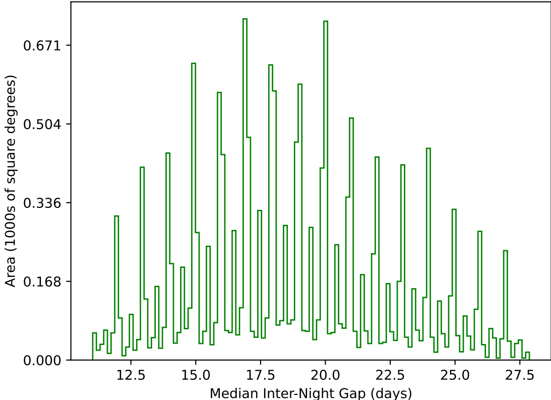
internal_u_expt45_nscale1.2v3.4_10yrs WFD g band: Median Inter-Night Gap
