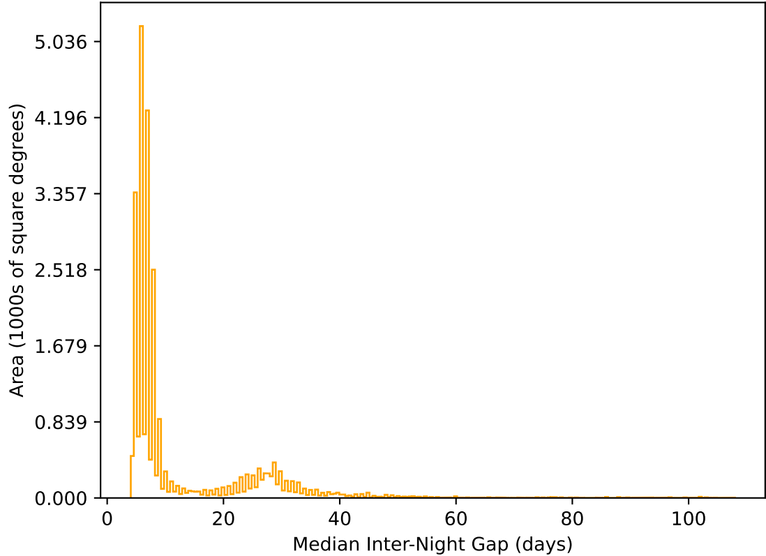
internal_u_expt45_nscale1.2v3.4_10yrs All sky r band: Median Inter-Night Gap
