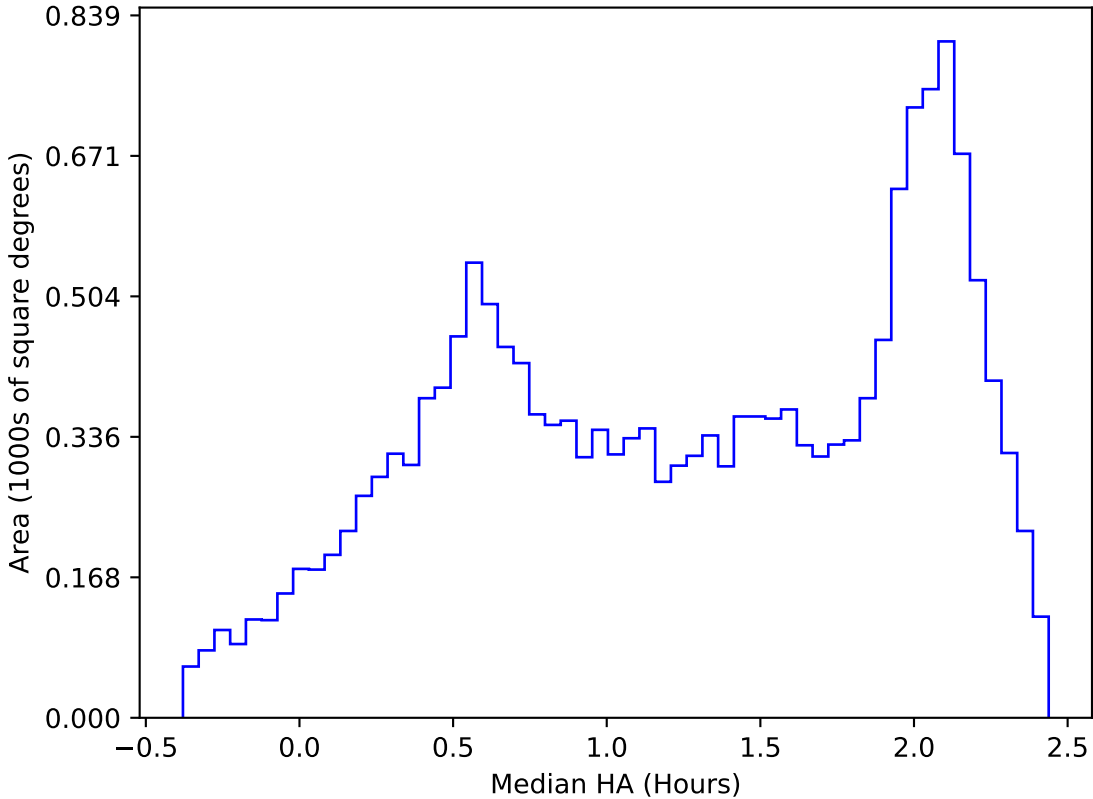
internal_u_expt45_nscale1.2v3.4_10yrs WFD y band: Median HA
