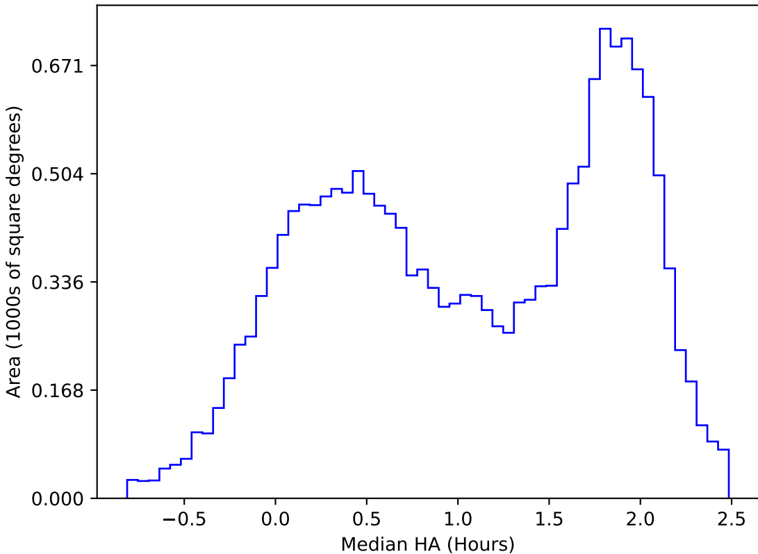
internal_u_expt45_nscale1.2v3.4_10yrs WFD u band: Median HA
