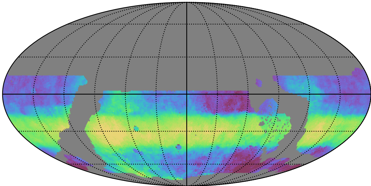
internal_u_expt45_nscale1.2v3.4_10yrs WFD r band: Median HA
