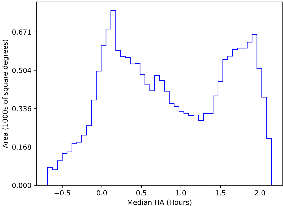
internal_u_expt45_nscale1.2v3.4_10yrs WFD r band: Median HA
