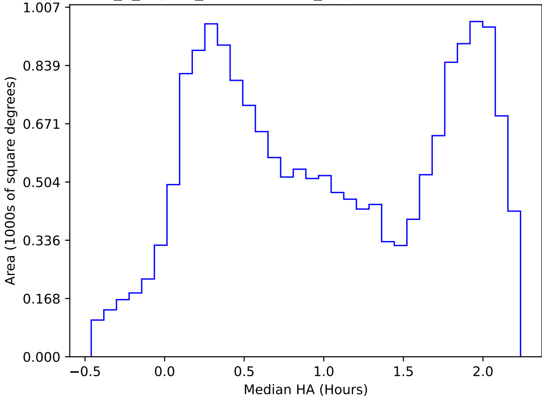
internal_u_expt45_nscale1.2v3.4_10yrs WFD i band: Median HA
